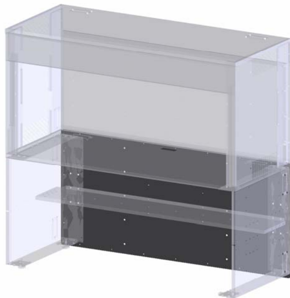
BACK PANEL FOR 72" FREE STANDING KIT PART# 50268
