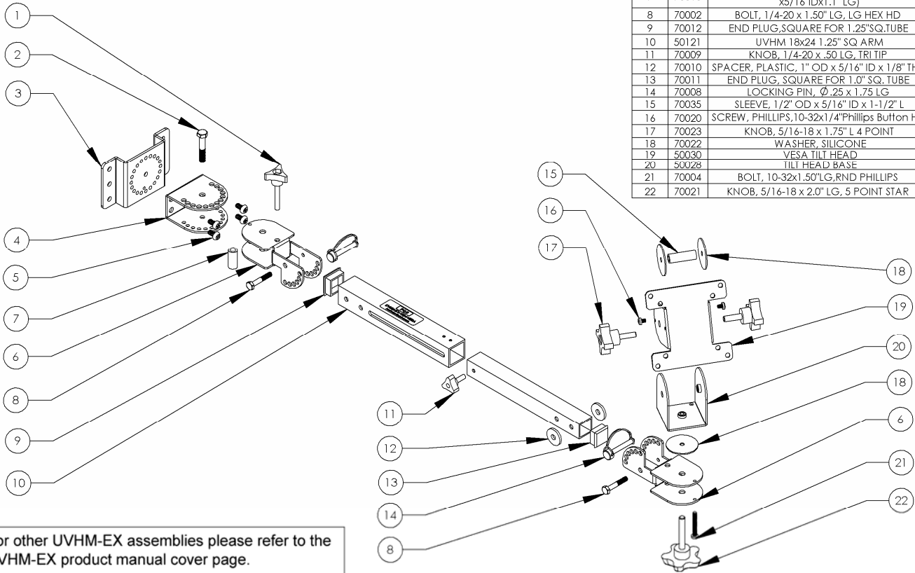
Figure 8 - EX Arm Mount
