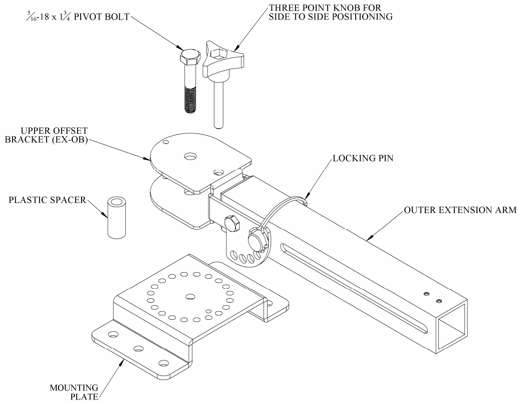
Figure 7 - EX Arm Mount outer extension arm assembly for flat mounting
