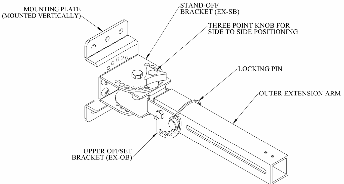
Figure 4 - EX Arm Mount with a P1 plate mounted in the vertical position
