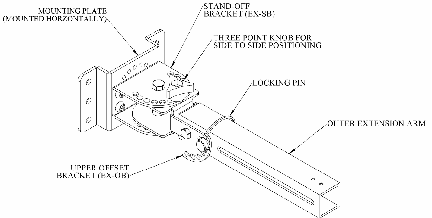
Figure 3 - EX Arm Mount with a P1 plate mounted in the horizontal position
