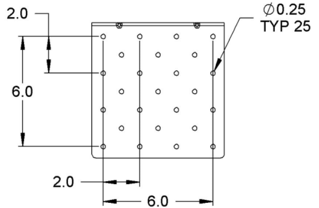
MOUNTING PLATE
