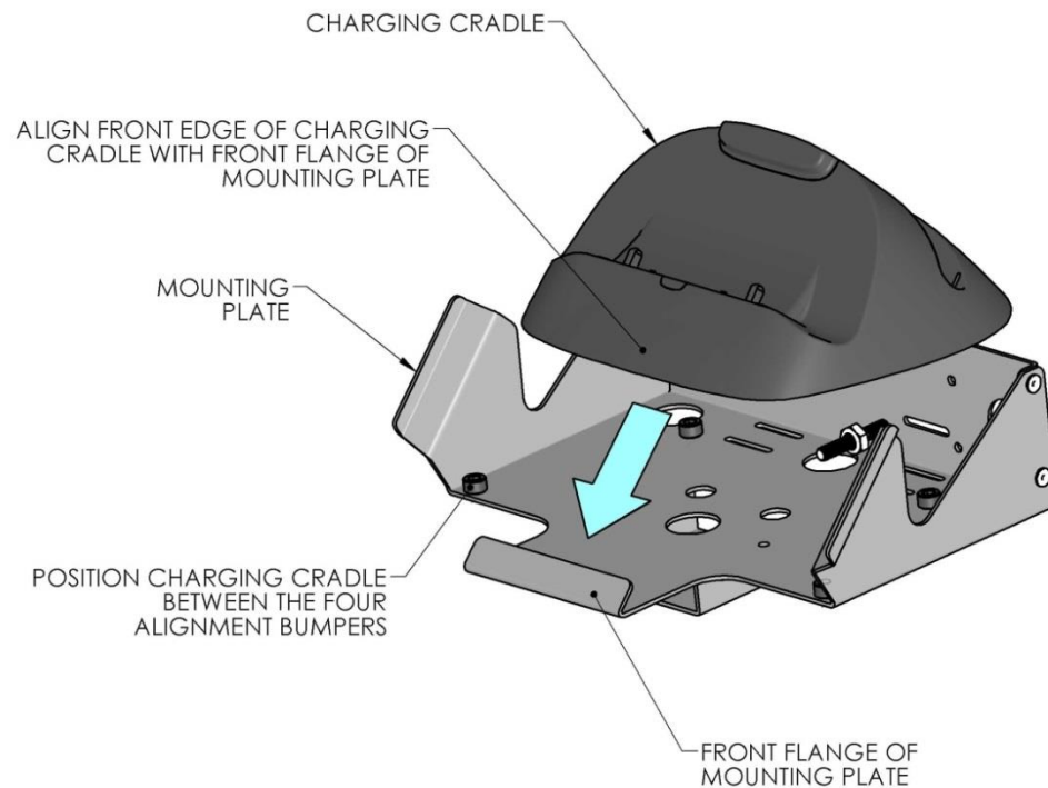
INSTALLATION DETAIL FOR ALL 505 SERIES MOUNTS WITH A DROP IN CHARGING CRADLE THAT PERMITS CONTINUOUS DAILY INSTALLATION AND REMOVAL OF THE TABLET
