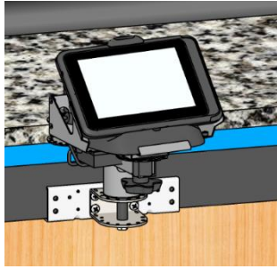
PN 80241-505 - Under Counter Mount with a 3" riser, adjustable 8" arm + panning head for a MICROS 720 Tablet with drop in charger
