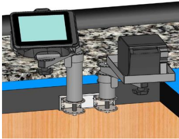
PN 80248-505 - Under Counter Mount with a 3" riser, a 6" riser, two adjustable 8" arms + panning heads for a MICROS 720 Tablet with drop in charger and a Flat Printer Tray
