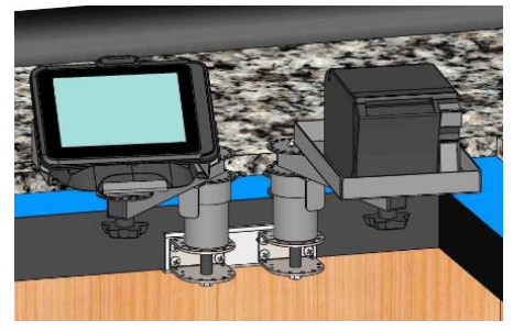
PN 80247-505 - Under Counter Mount with two 3" risers, two adjustable 8" arms + panning heads for a MICROS 720 Tablet with drop in charger and a Flat Printer Tray
