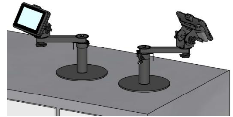
PN 80623-504 - Countertop Movable Pedestal Mount with a 6" riser, adjustable 8" arm + pan and tilt head for semi-permanent support of a MICROS 720 Tablet
