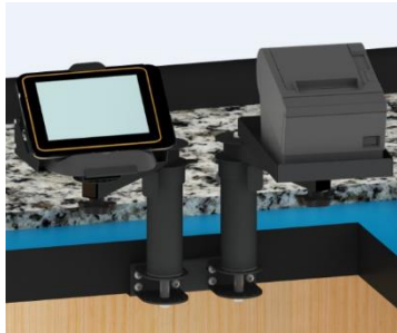
PN 80246-505 - Under Counter Mount with two 6" risers, two adjustable 8" arms + panning head for a MICROS 720 Tablet with drop in charger + a Flat Printer Tray
