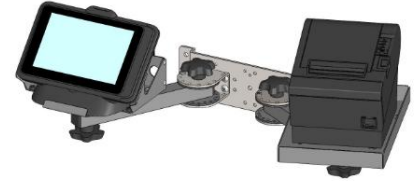
PN 80003-505 - Wall Mount + two adjustable 8" arms + panning heads for a MICROS 720 Tablet with drop in charger and a Flat Printer Tray
