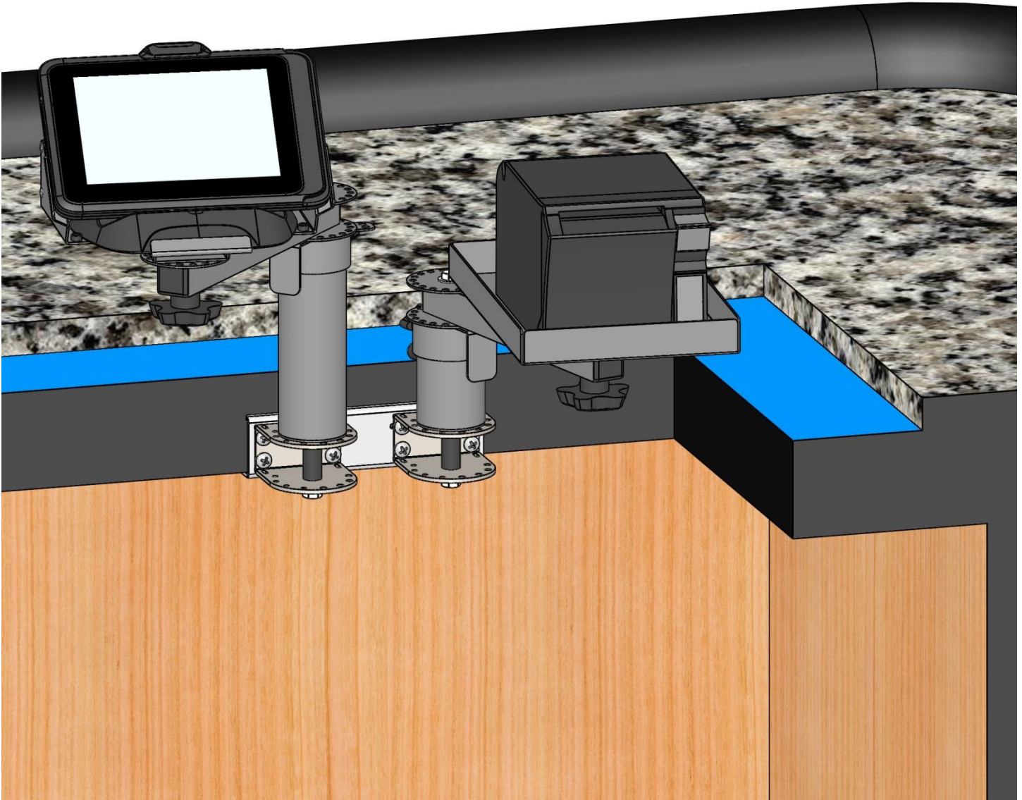
PN 80248-505 with 1-3" Riser + 1-6" Riser
