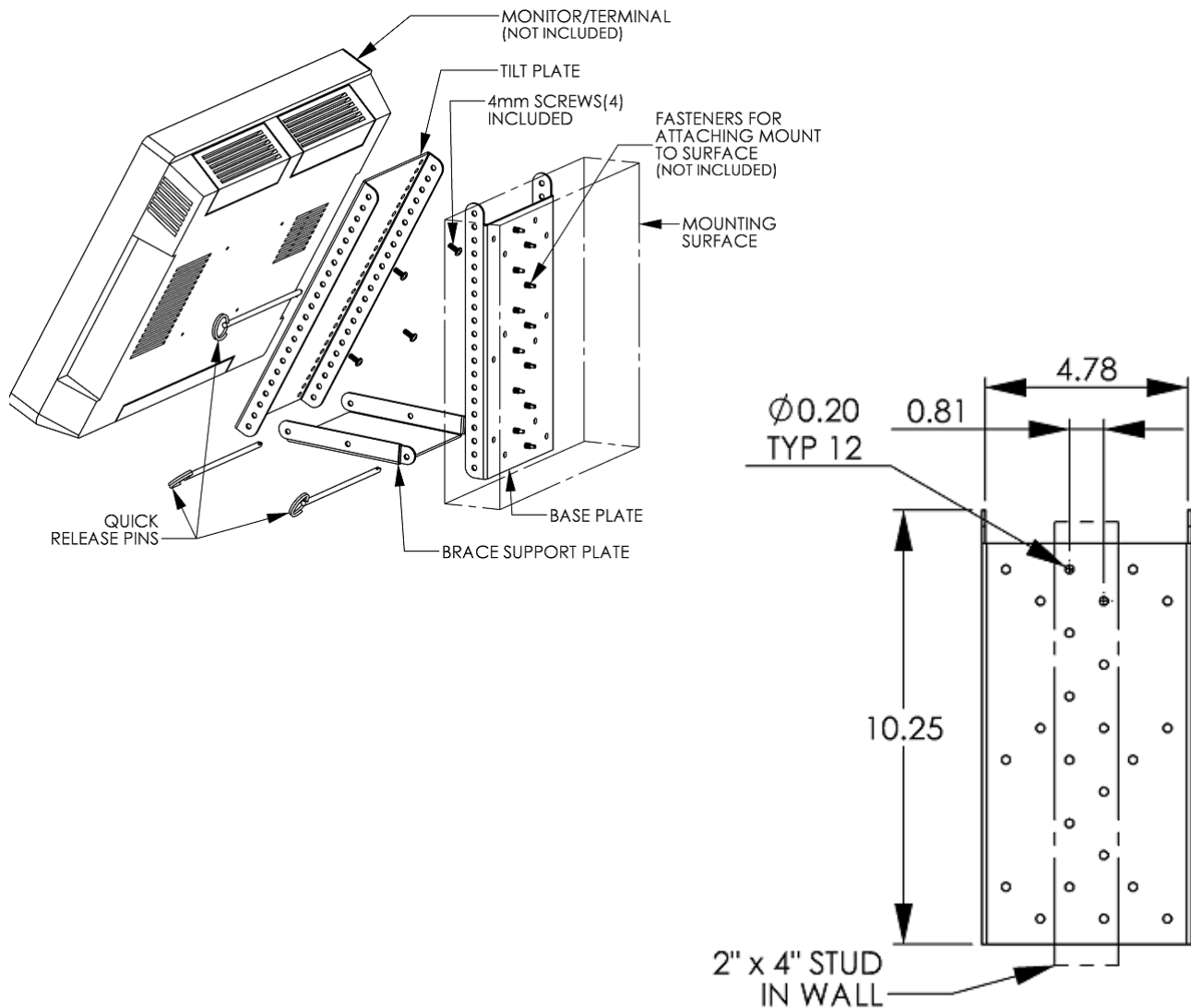
WALL MOUNTING PLATE
