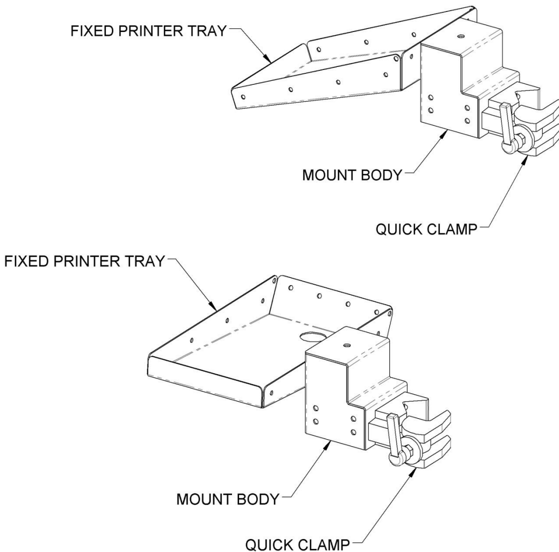
Alternate tray mounting configuration
