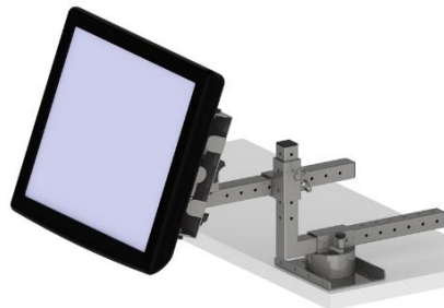
PN 90290 - Fully Articulated Shelf Edge KDS Support Package for a VESA Touchscreen and any Controller
