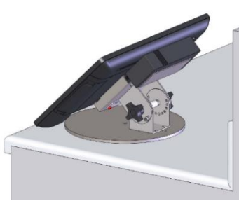
PN 80622-MICROS - Countertop Movable Pedestal Mount + WS6 Pan - Tilt Head + PS holder
