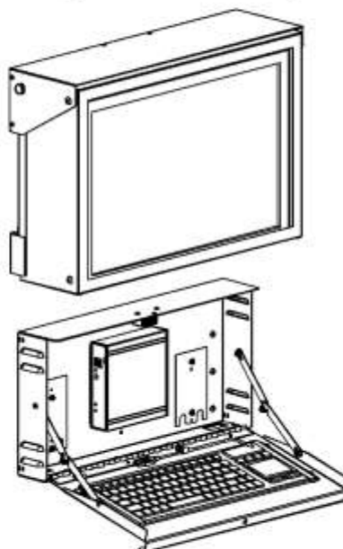
WALL MOUNT ENCLOSURE WITH AN ALL IN ONE KEYBOARD SHOWN WITH A UNIVERSAL MONITOR ENCLOSURE AND A THIN CLIENT P/N : 80682
