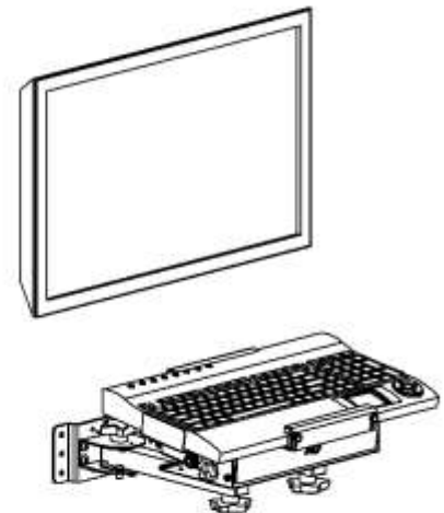
UNIVERSAL WALL MOUNTED ADJUSTABLE KEYBOARD TRAY ON TWO ARMS P/N : 80010
