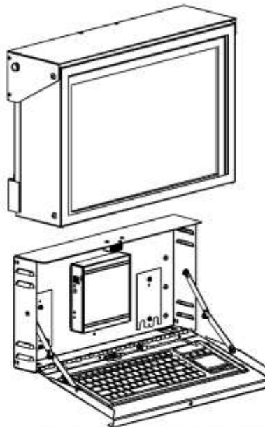
WALL MOUNT ENCLOSURE WITH AN ALL IN ONE KEYBOARD SHOWN WITH A UNIVERSAL MONITOR ENCLOSURE AND A THIN CLIENT P/N : 80682
