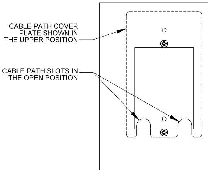
REAR CABLE PATH PLATE DETAIL
