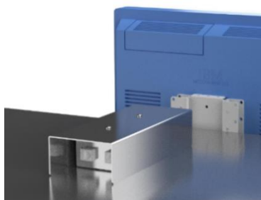
PN 80540 - Low Profile Data Outlet with Heat Shield
