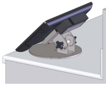
PN 80622-MICROS - Countertop Movable Pedestal Mount + WS6 Pan - Tilt Head + PS holder
