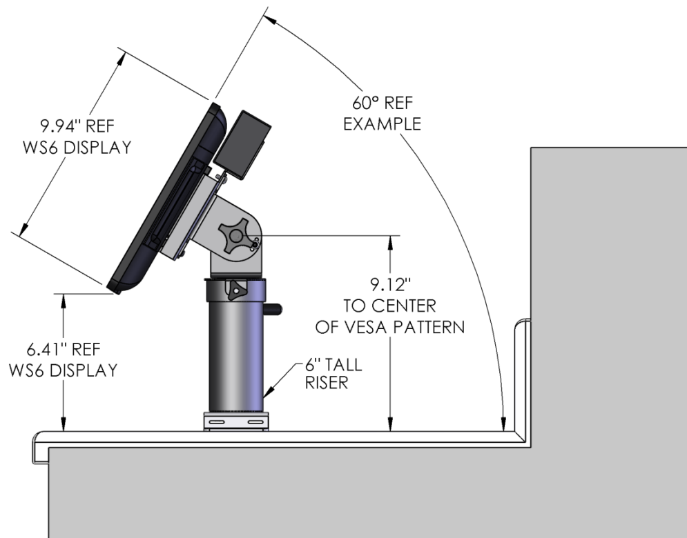
PN 80100-MICROS 6" Riser
