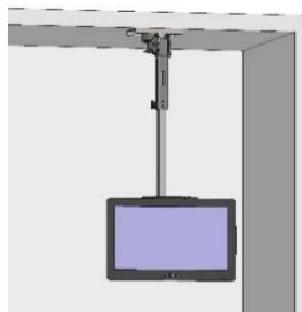
PN 80104-2026-MICROS - 7 Axis Ceiling Mount + 20" Extendable Arm + Biased WS6 Pan - Tilt Head + PS holder
